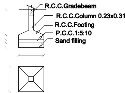
Foundation details
