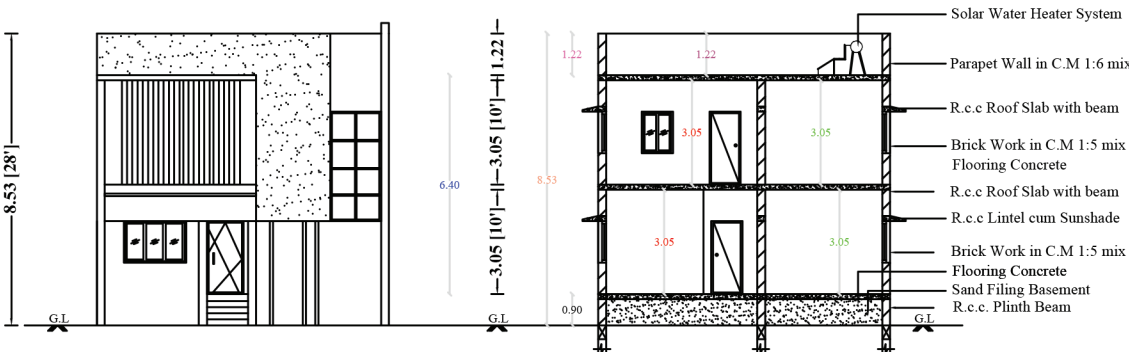
FRONT ELEVATION
