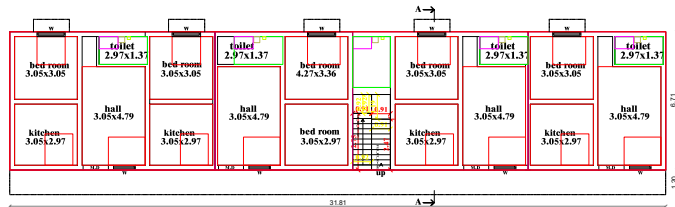
PRO. FIRST FLOOR PLAN
