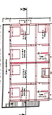
BLOCK 2 - FIRST FLOOR PLAN
