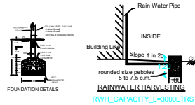
RAINWATER HARVESTING
