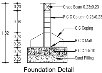
Foundation Detail
