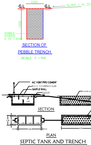
SEPTIC TANK AND TRENCH
