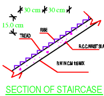
SECTION OF STAIRCASE
