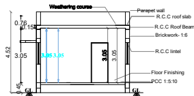
SECTION ON 'AA'
