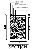
RAIN WATER HARVESTING PERCOLATION BED
