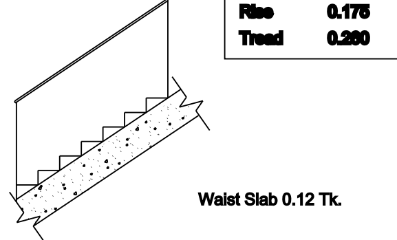
Staircase Details
