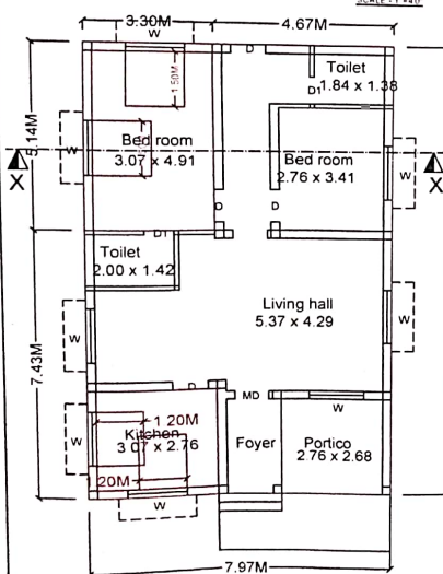
EXISTING CUM PROPOSED GROUND FLOOR PLAN
