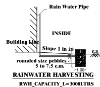
SECTION ON 'AA'
