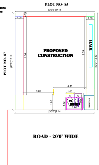
SITE PLAN - SCALE (1:100)
