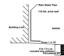
PERCOLATION PIT
