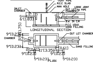
SEPTIC TANK:
