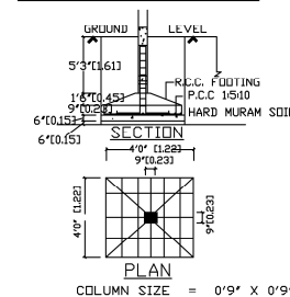
FOUNDATION DETAILS
