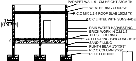
CROSS SECTION ON "AB"
