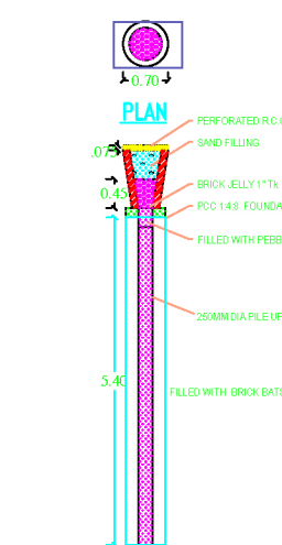
PERCOLATION PIT SECTION OF RAIN WATER RWH CAPACITY L=3.76
