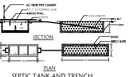
PLAN SEPTIC TANK AND TRENCH
