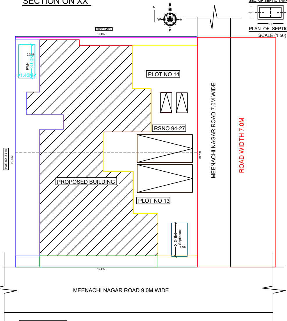
SITE PLAN
