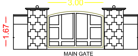
MAIN GATE
