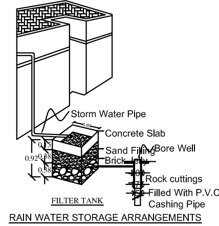
RAIN WATER STORAGE ARRANGEMENTS
