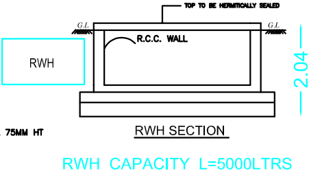
RWHP_CAPACITY_L=5000LRS
