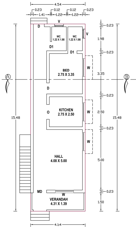
PRO.GROUND FLOOR
