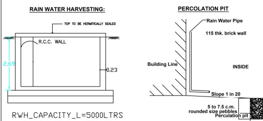
PERCOLATION PIT
