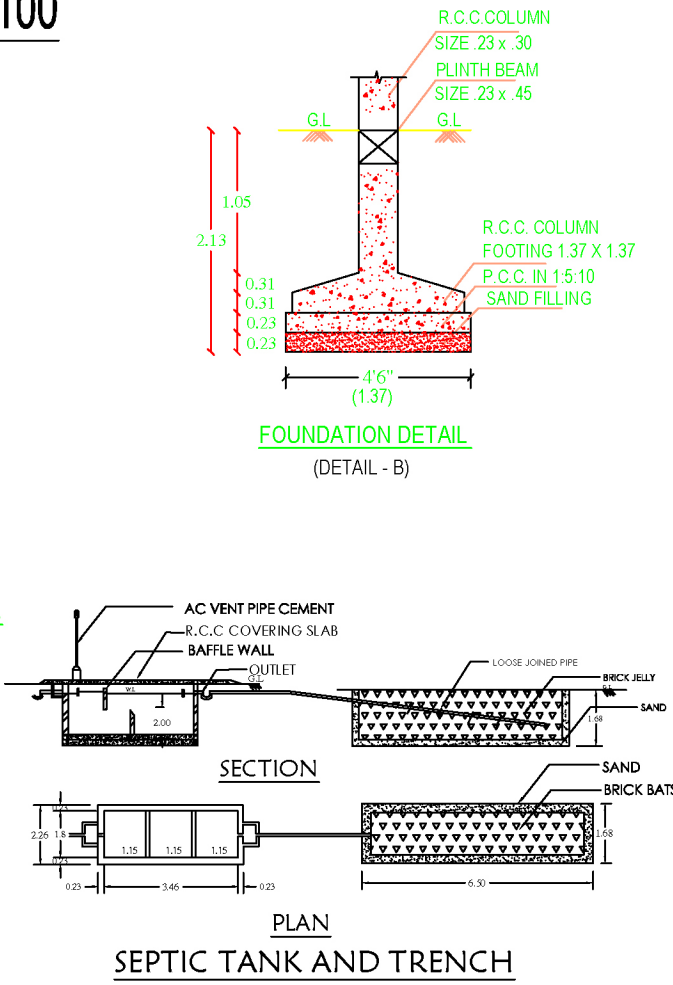
SEPTIC TANK AND TRENCH
