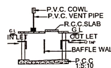
SEC. OF SEPTIC TANK
