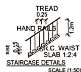
STAIRCASE DETAILS SCALE (1:50)
