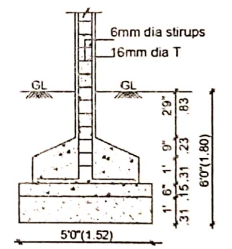
COLUMN FOUNDATION DETAIL SCALE (1:50)
