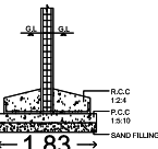
COLUMN DETAILS [ NOT TO SCALE ]
