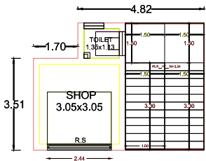
PRO.GROUND FLOOR PLAN
