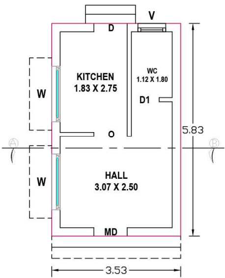
PRO.GROUND FLOOR
