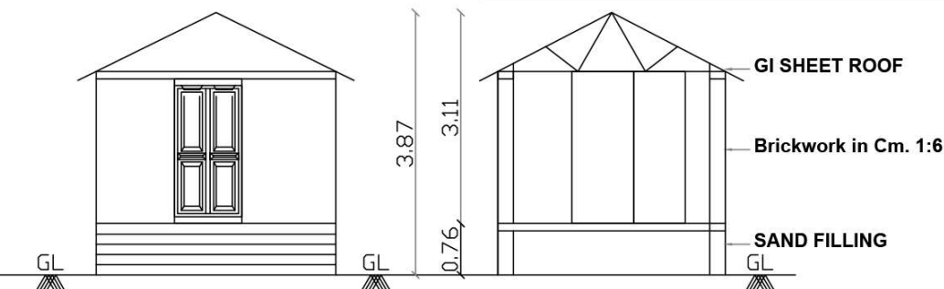
FRONT ELEVATION
