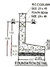
FOUNDATION DETAIL
