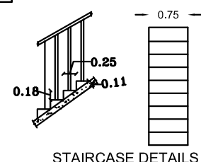
STAIRCASE DETAILS
