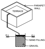
COLLECTION SUMP FOR HARVESTING FOR TERRACE
