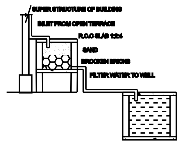
RAINWATER HARVESTING
