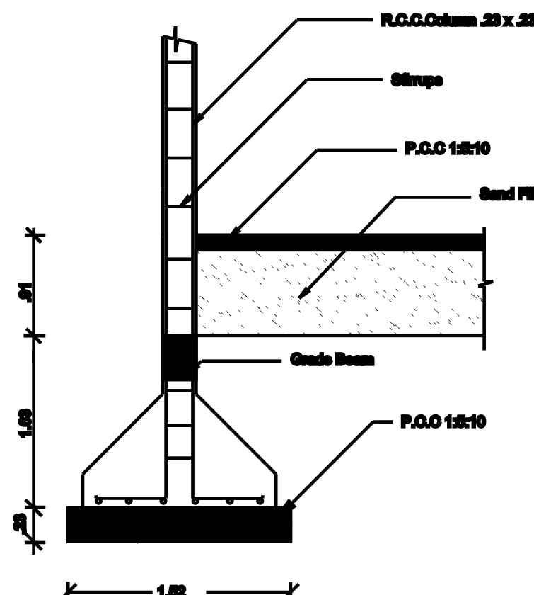
COLUMN DETAIL
