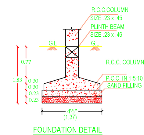
FOUNDATION DETAIL
