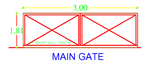
MAIN GATE
