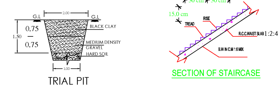
TRIAL PIT
