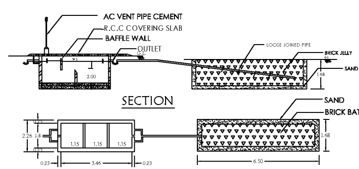
SEPTIC TANK AND TRENCH
