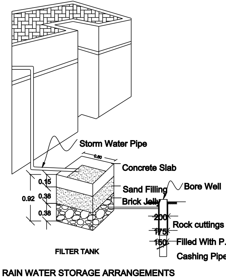
RAIN WATER STORAGE ARRANGEMENTS
