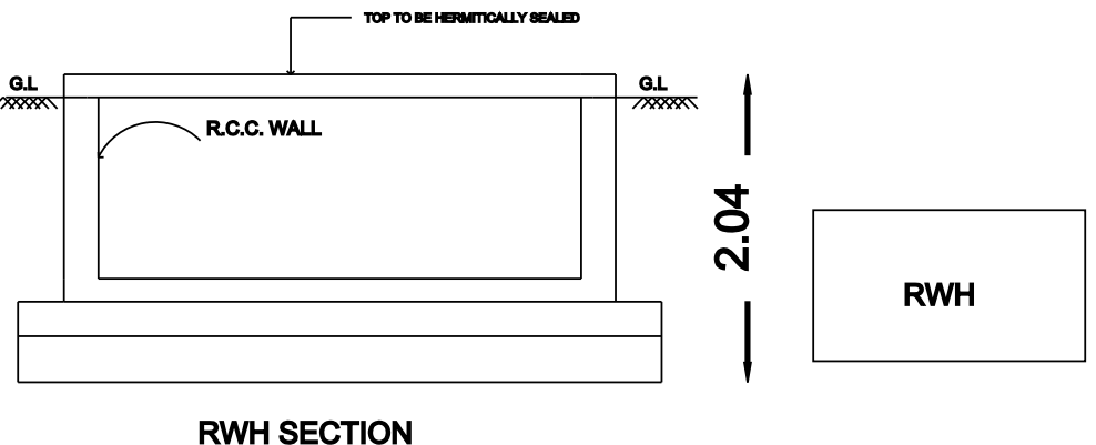
RWH SECTION
