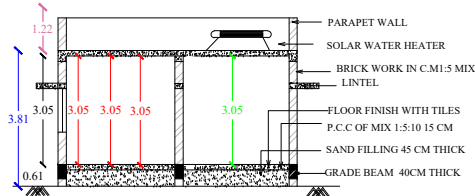
SECTION- AA1
