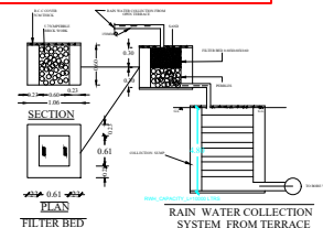
RAIN WATER COLLECTION SYSTEM FROM TERRACE
