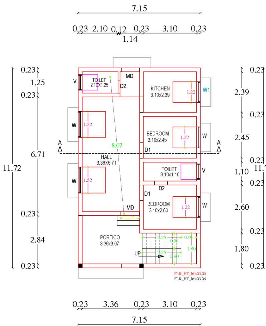
FLOOR PLAN
