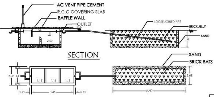
SECTION SEPTIC TANK AND TRENCH
