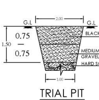
TRIAL PIT
