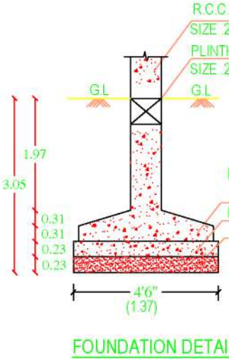
FOUNDATION DETAIL
