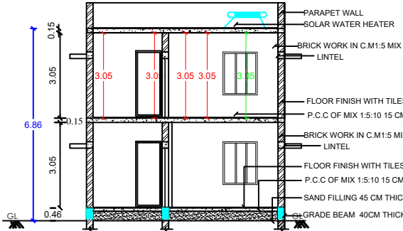
SECTION-AB
