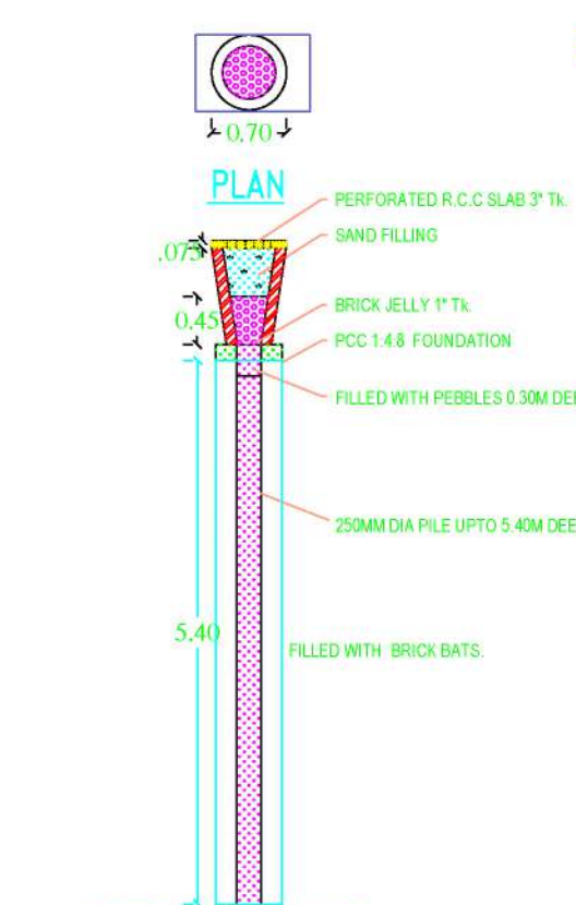
PERCOLATION PIT SECTION OF RAIN WATER
