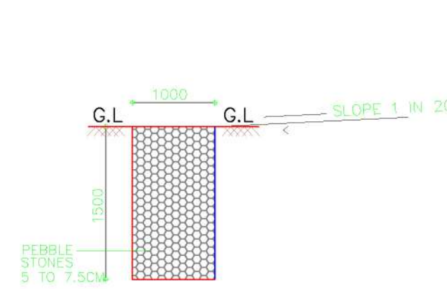
PEBBLE TRENCH SCALE : 1: = 100
