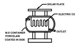
SOLAR SYSTEM
