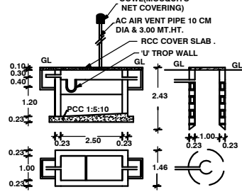
PLAN AND CROSS SECTION OF ST&SP.
