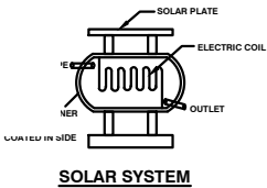
SOLAR SYSTEM
