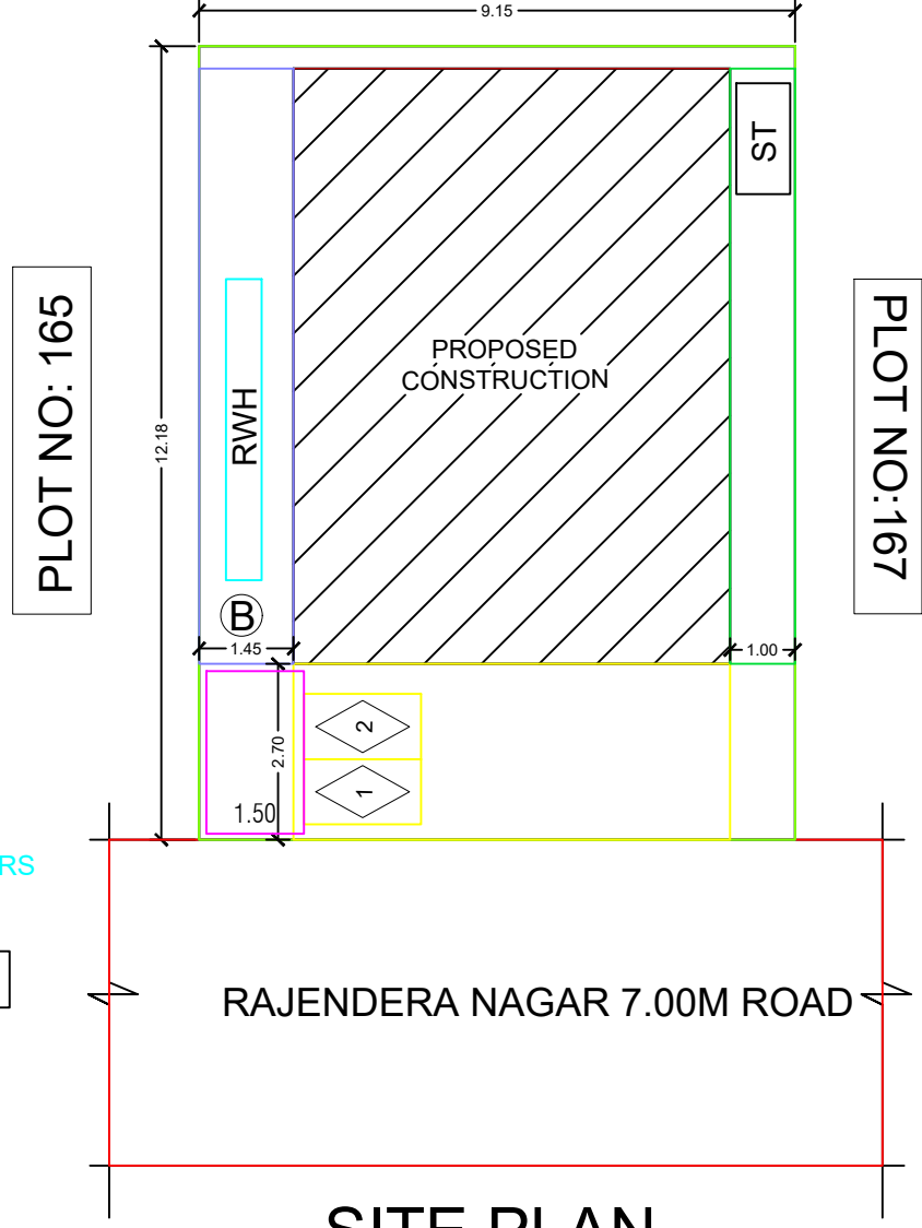
SITE PLAN
