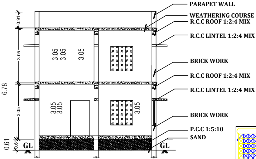
SECTION ON - "SP"
