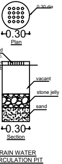
RAIN WATER PERCOLATION PIT
