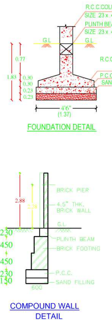
FOUNDATION DETAIL
