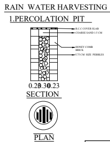
RAIN WATER HARVESTING L.PERCOLATION PIT
