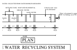
WATER RECYCLING SYSTEM
