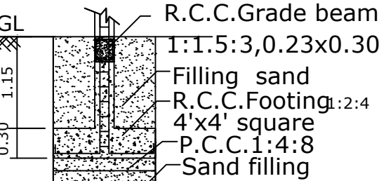
Foundation details
