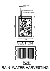
RAIN WATER HARVESTING PERCOLATION BED
