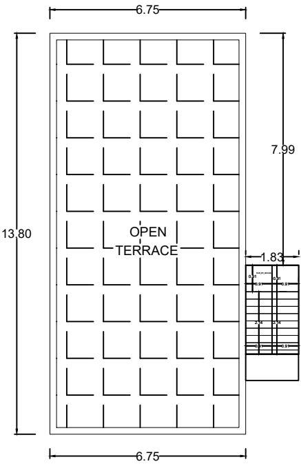
PRO.TERRACE FLOOR PLAN
