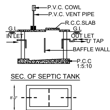
PLAN OF SEPTIC TANK SCALE (1:50)
