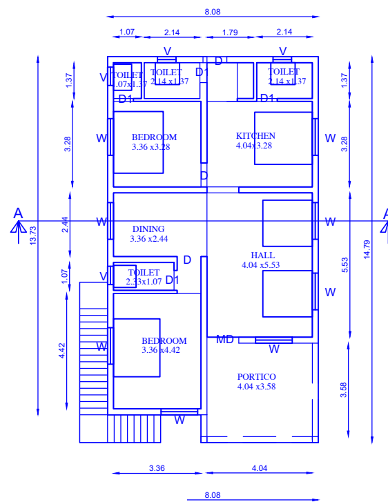
FLOOR PLAN
