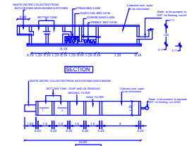
WASTE WATER RECYCLING SYSTEM
