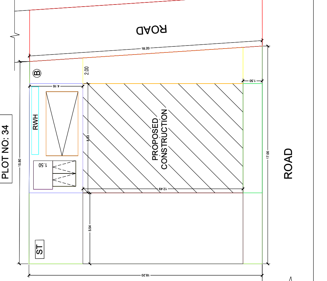
SITE PLAN (1:100)
