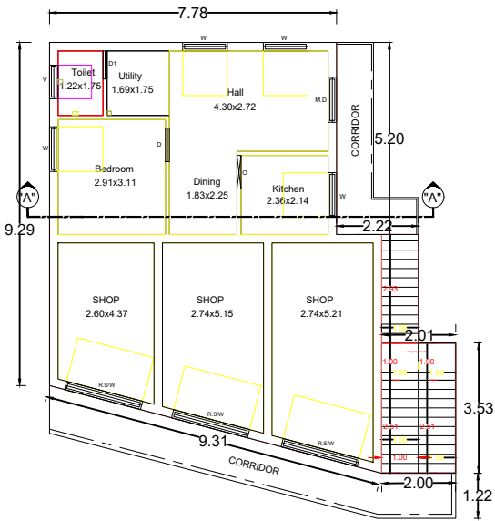
PRO.FIRST FLOOR PLAN
