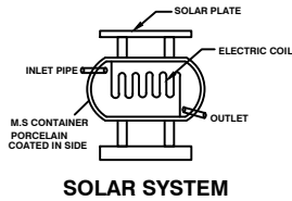
SOLAR SYSTEM
