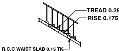
STAIR CASE DETAILS
