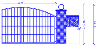
COMPOUND GATE (NOT TO SCALE)
