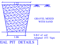
TRIAL PIT DETAILS
