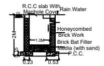
Details of Rain Water Collection (Recharge Well) Member Scale: 1:50
