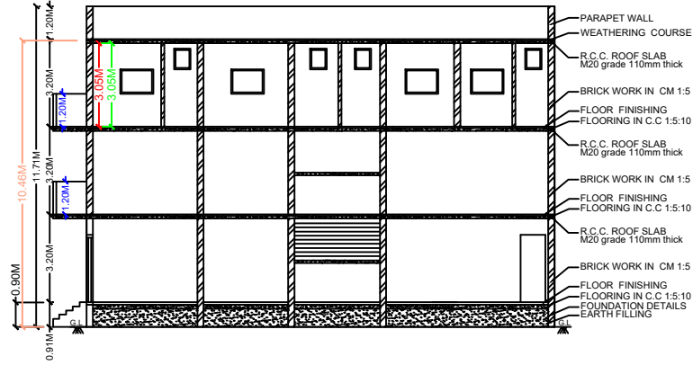
SECTION ON XX
