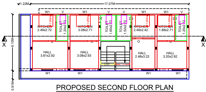
PROPOSED SECOND FLOOR PLAN
