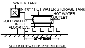
SOLAR HOT WATER SYSTEM DETAIL
