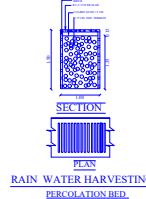
PLAN RAIN WATER HARVESTING PERCOLATION BED.
